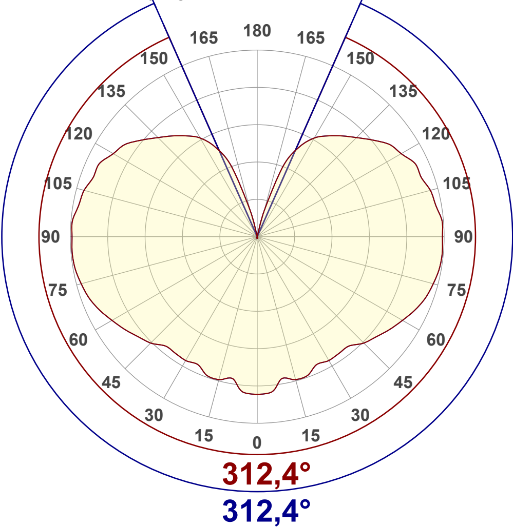
Luminous Intensity diagram
